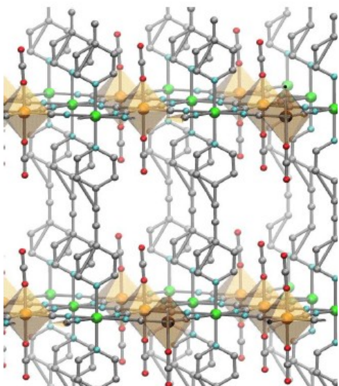
Figure 1: Crystal structure of M(bpac)M'(CN)_4 with CO 2 molecules adsorbed at the apical sites of the 4-fold coordinated metal M.
